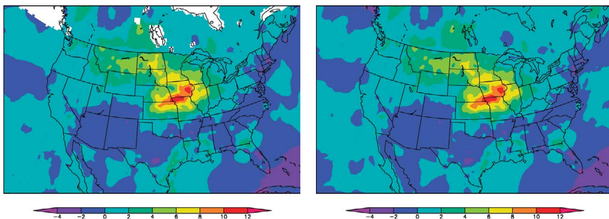
FIG. 4. Difference between 1993 and 1988 of the monthly average precipitation over June–July (in. month -1 ) for (left) the observed precipitation, assimilated by the NARR over land and over low- and lower midlatitude oceans, and (right) the NARR precipitation.
