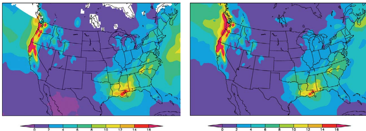
FIG. 3. (left) Observed (analyzed) precipitation assimilated by the NARR over land and over low- and lower midlatitude oceans and (right) NARR precipitation, averaged for January 1998 (in. month -1 ). White indicates no available observations.
